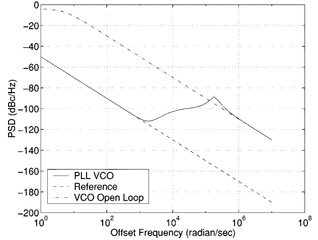
Fig. 2. PSD of the PLL output with no loop filter.
