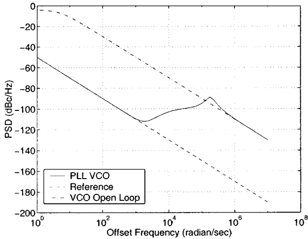
Fig. 5. CPPLL spectrum (second-order loop filter).
