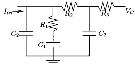
Fig. 6. Loop filter reported in [23].
