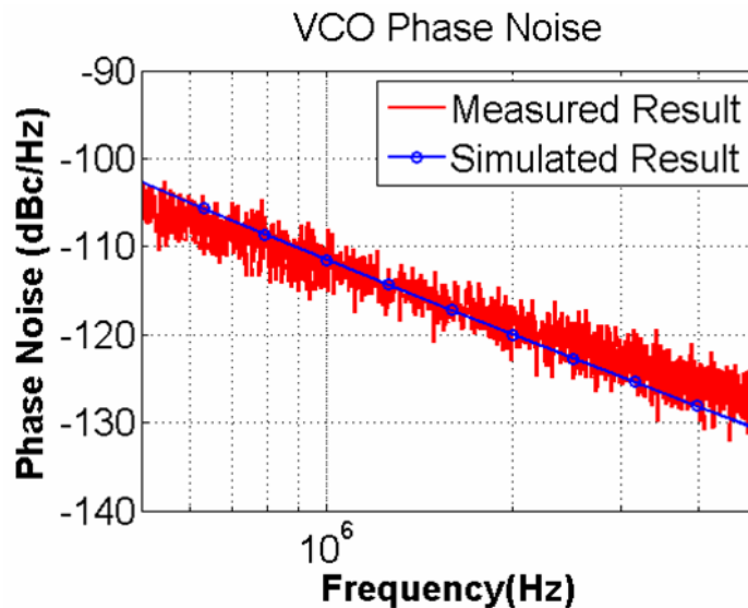
Figure 2: Comparison of simulated to measured phase-noise of the LC-VCO
