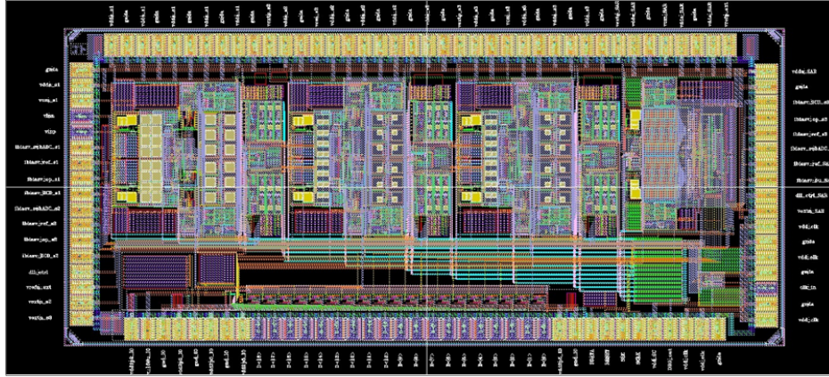
Figure 3: Pipeline ADC chip layout
