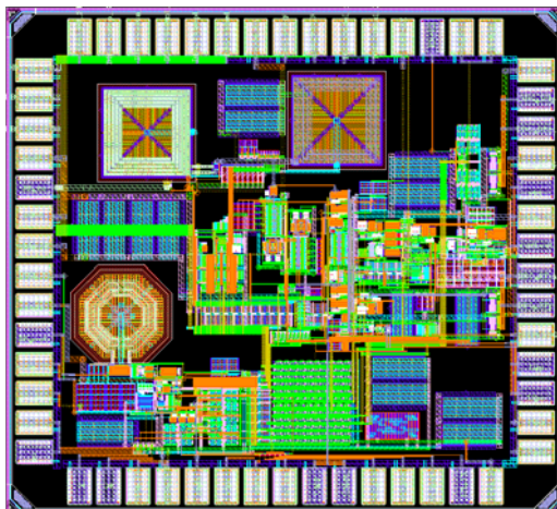
Figure 4: Ultra-wideband transceiver chip layout
