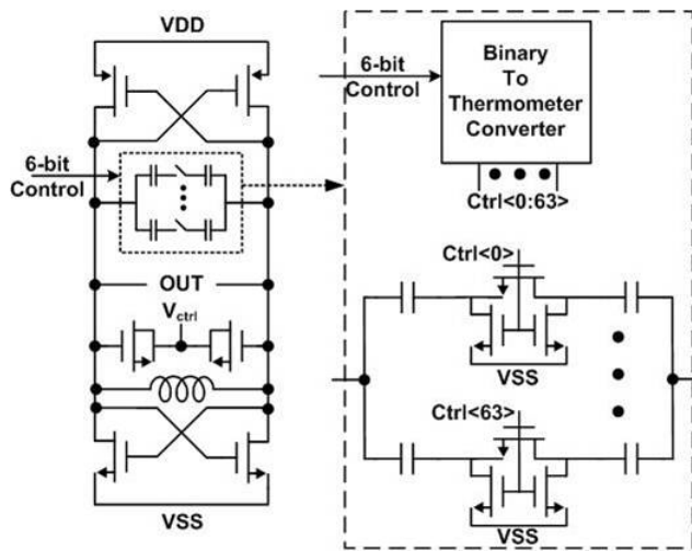
Figure 1 Circuit implementation of the LC-VCO
